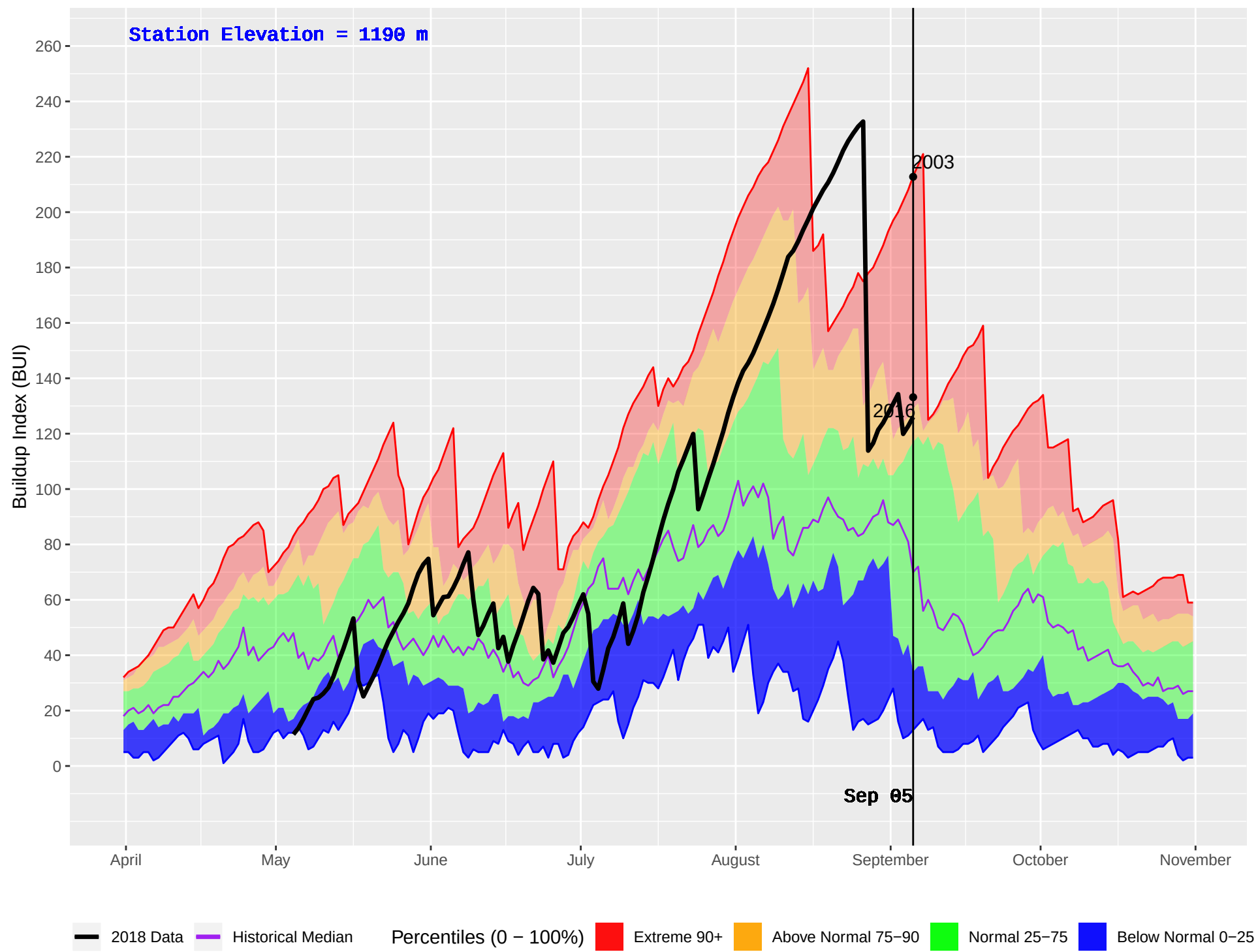
EMILY CREEK (425) : Historical (2002–2016) and Current (2018) Daily Buildup Index (BUI)
