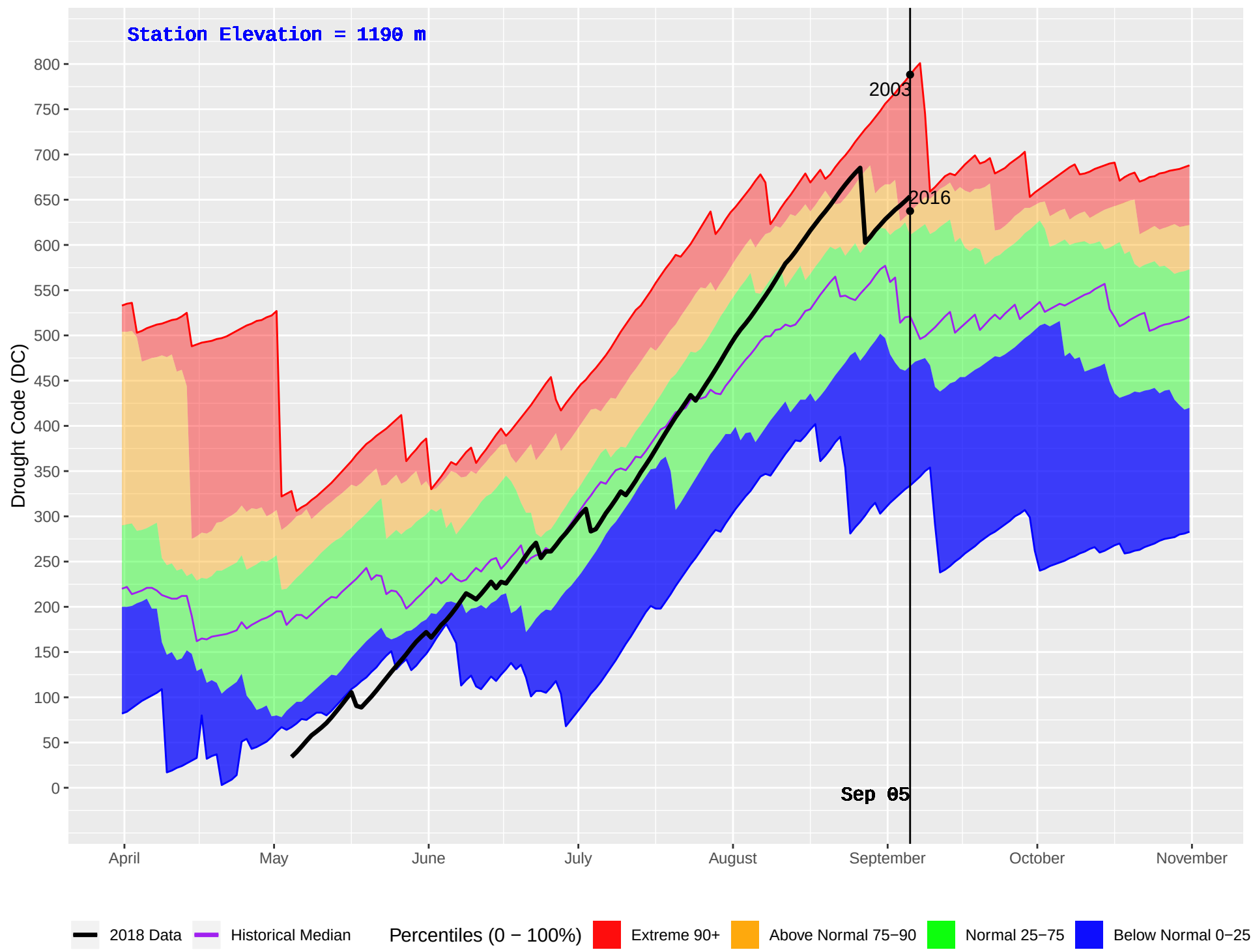
EMILY CREEK (425) : Historical (2002–2016) and Current (2018) Daily Drought Code (DC)
