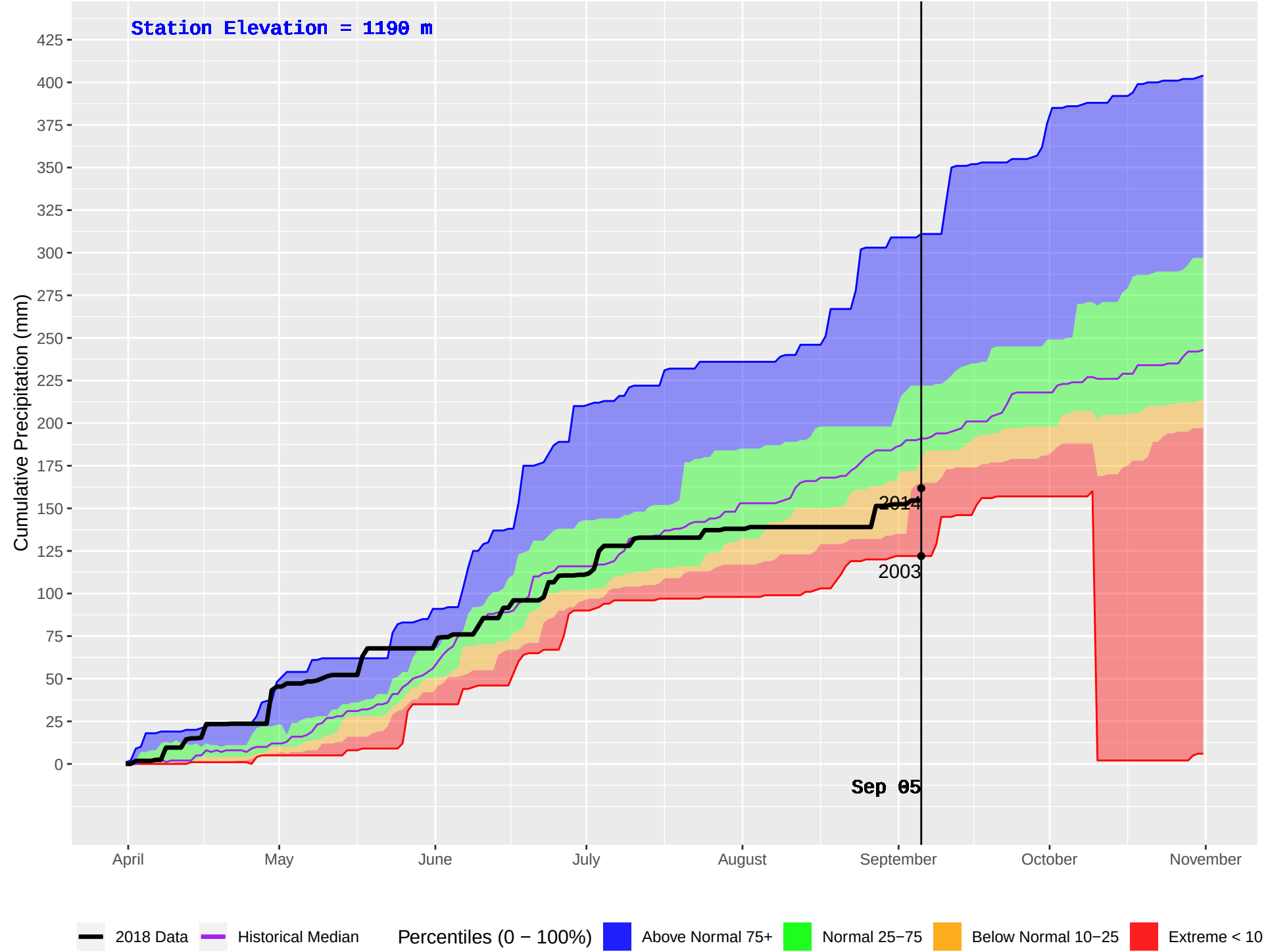
EMILY CREEK (425) : Historical (2002–2016) and Current (2018) Daily Cumulative Precipitation
