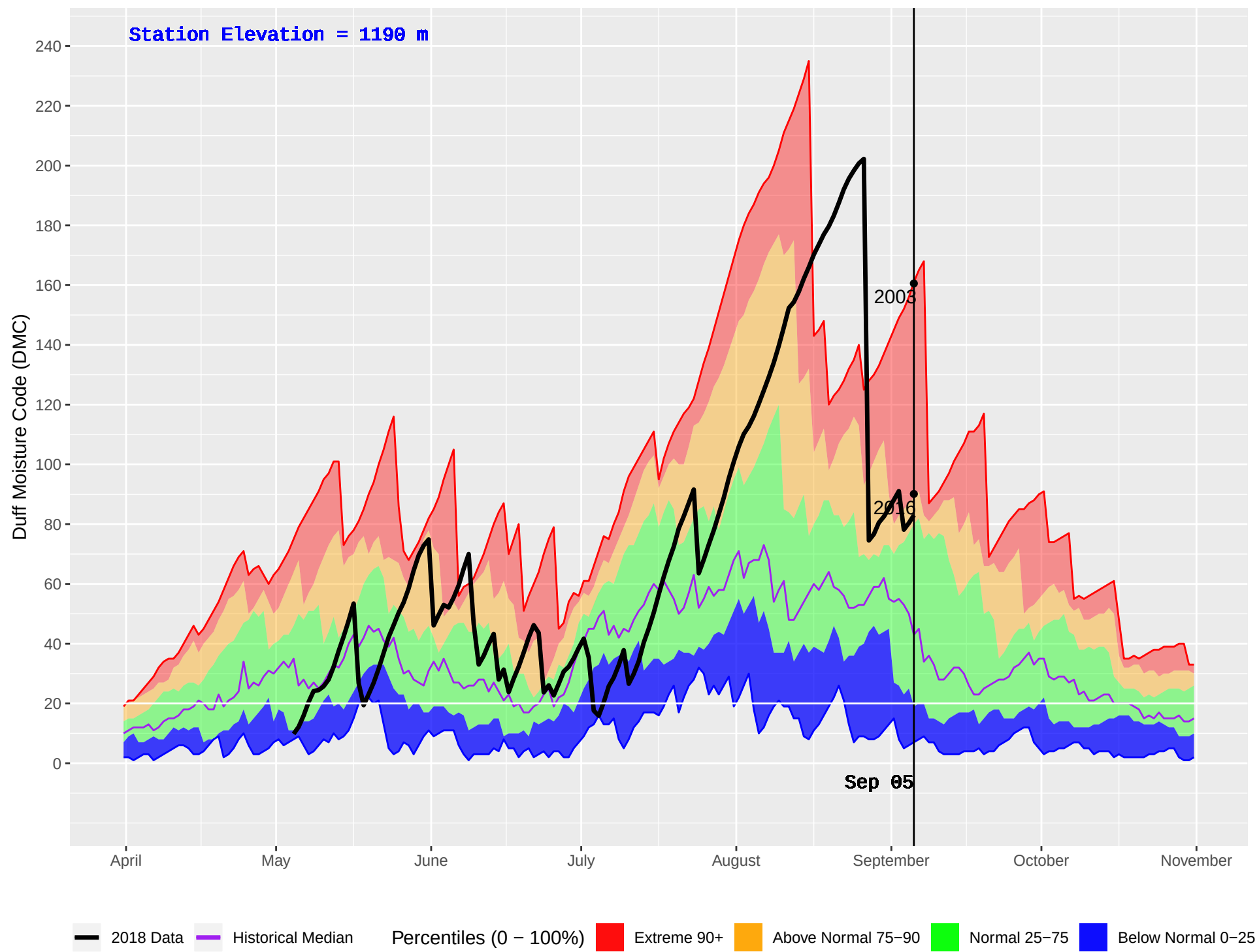
EMILY CREEK (425) : Historical (2002–2016) and Current (2018) Daily Duff Moisture Code (DMC)
