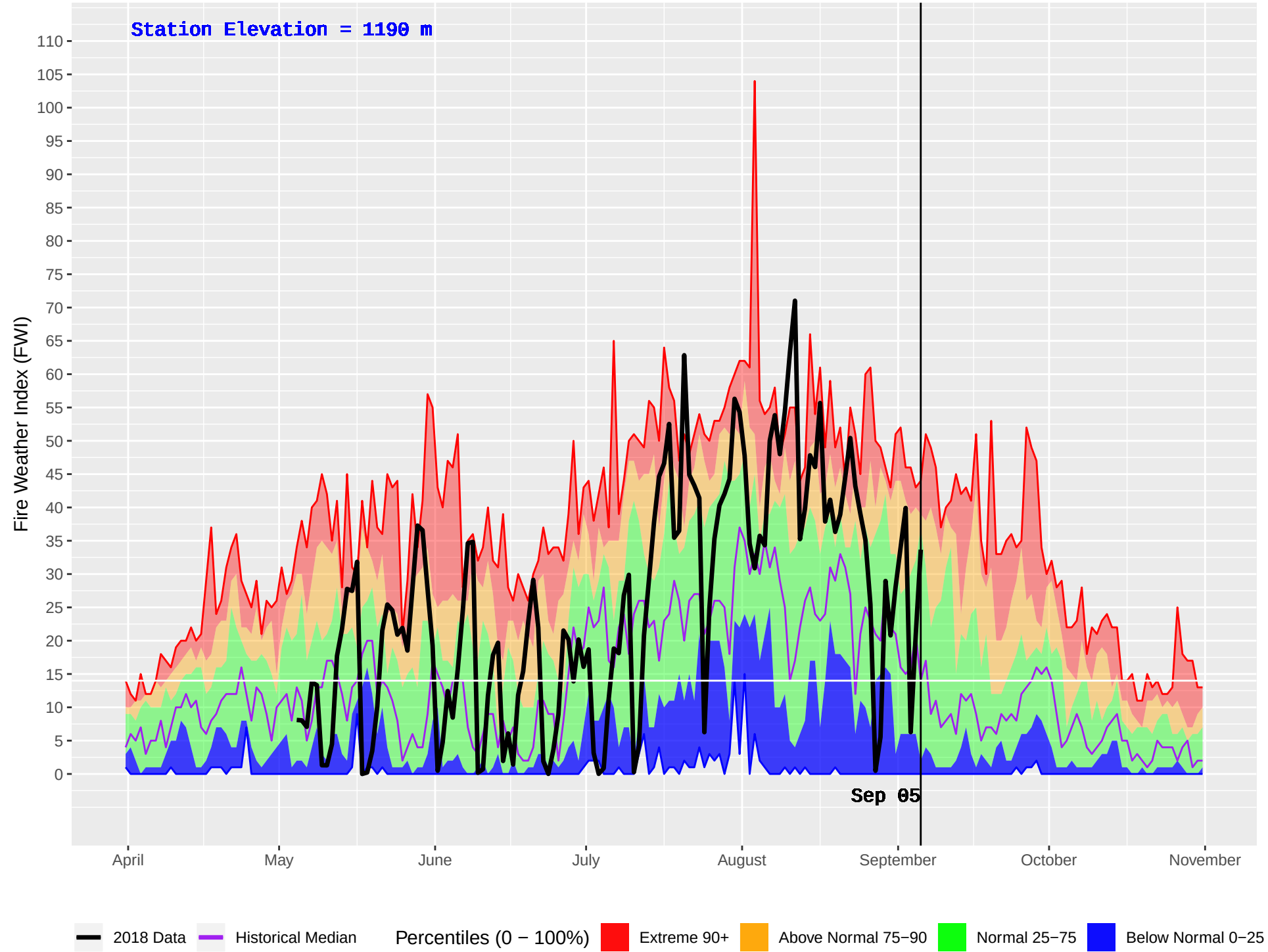
EMILY CREEK (425) : Historical (2002–2016) and Current (2018) Daily Fire Weather Index (FWI)
