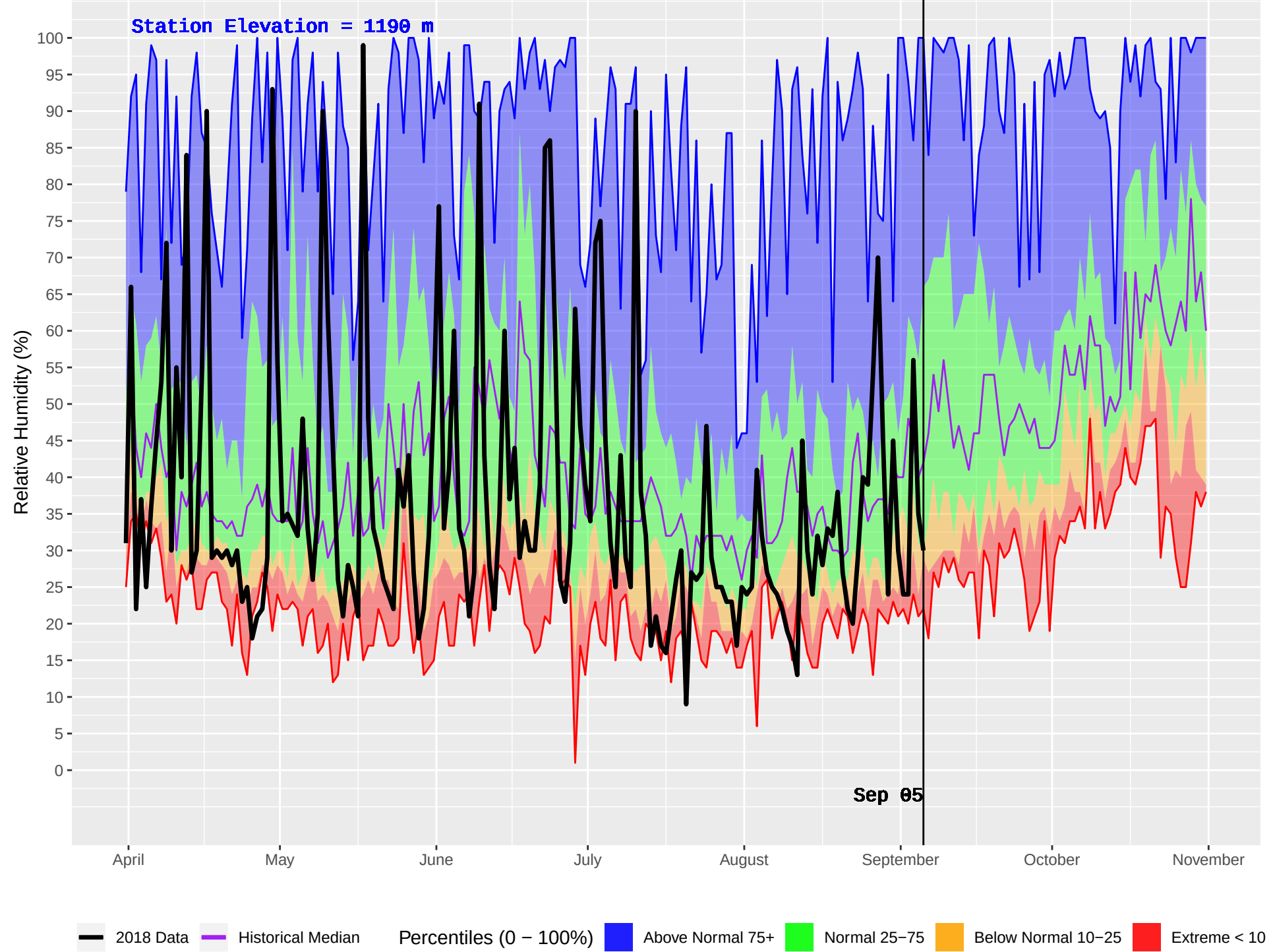
EMILY CREEK (425) : Historical (2002–2016) and Current (2018) Daily Relative Humidity
