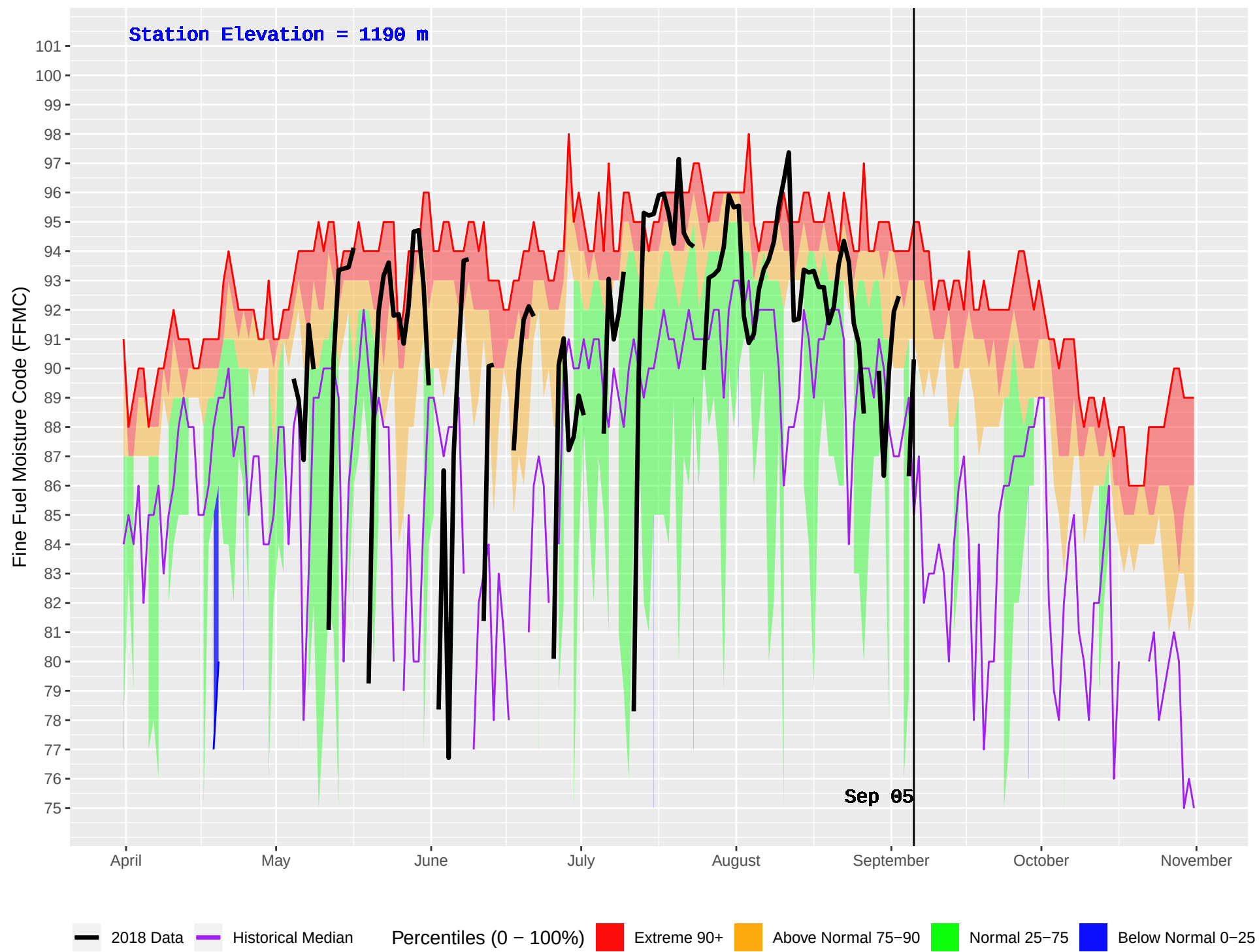
EMILY CREEK (425) : Historical (2002–2016) and Current (2018) Daily Fine Fuel Moisture Code (FFMC)
